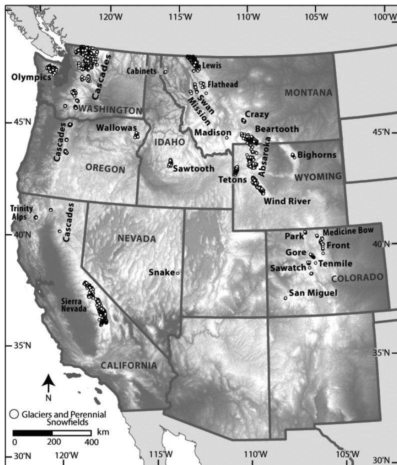
FIGURE 2. Distribution of G&PS in the American West (circles) with names of glacier-populated mountain ranges.
