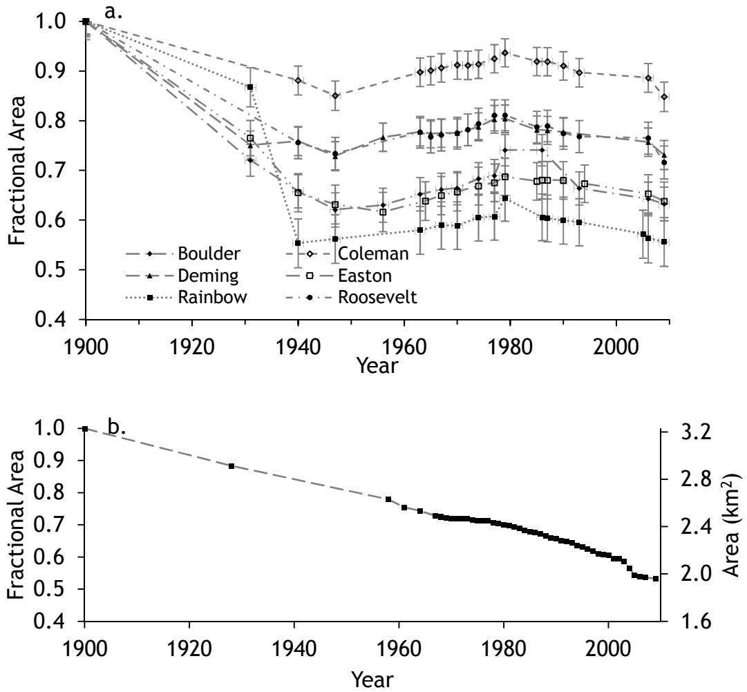
Figure 18 - Area change for glaciers on Mount Baker (a) and South Cascade Glacier (b).
